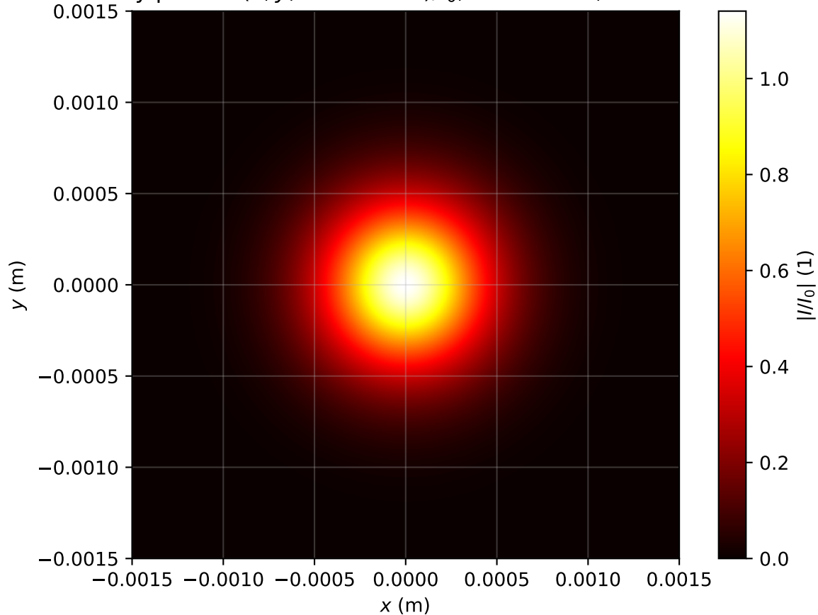
Intensity profile I(x, y, z = 0.557m)/I_0 , \text{Pin}=0.8\text{Pcr} , artificial time
